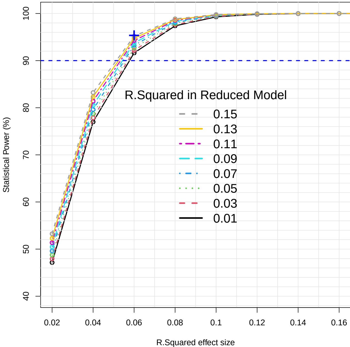
Aim 1a & 1b: Attained statistical power by effect size for various R.Squared values
