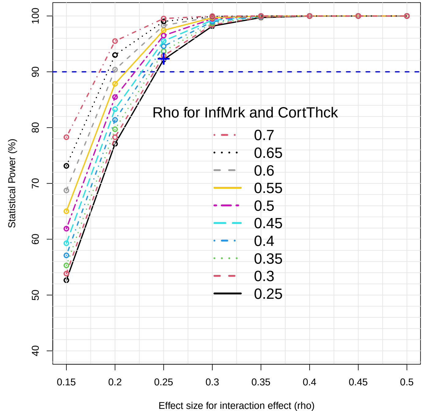
Aim 2: Attained statistical power by interaction effect size for various rho between predictor and outcome
